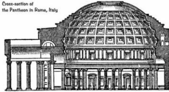
Cross-section of the Pantheon in Rome, Italy
